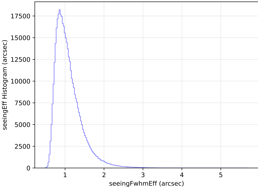
internal_u_expt38_nscale1.5v3.4_10yrs All sky z band: seeingEff Histogram
