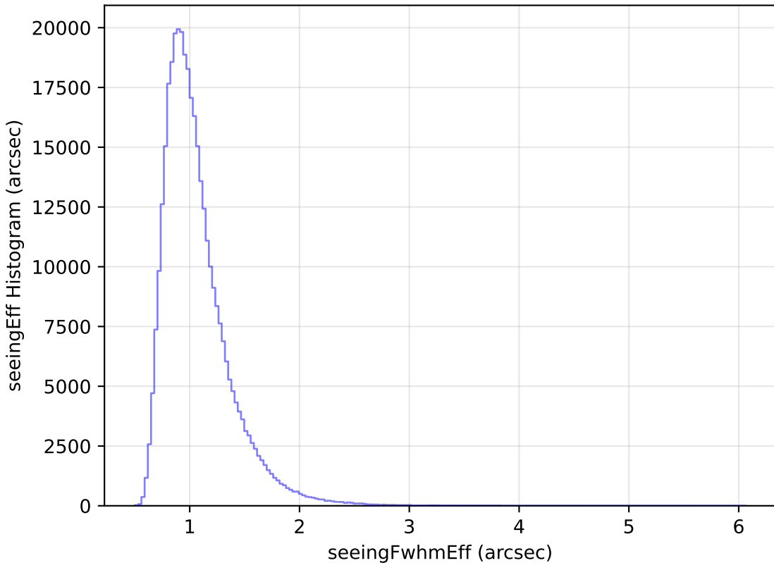
internal_u_expt38_nscale1.5v3.4_10yrs All sky y band: seeingEff Histogram
