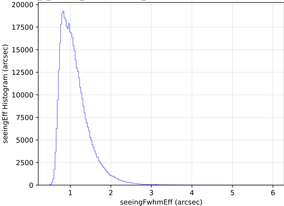
internal_u_expt38_nscale1.5v3.4_10yrs All sky r band: seeingEff Histogram
