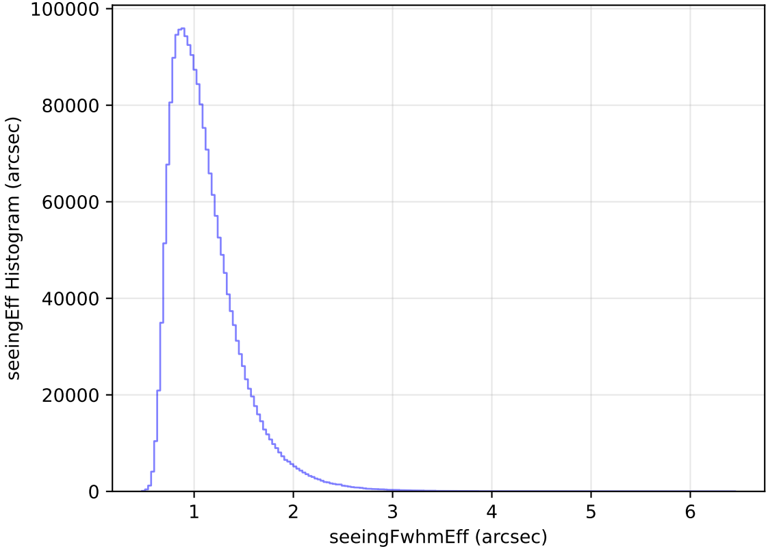
internal_u_expt38_nscale1.5v3.4_10yrs All sky all bands: seeingEff Histogram
