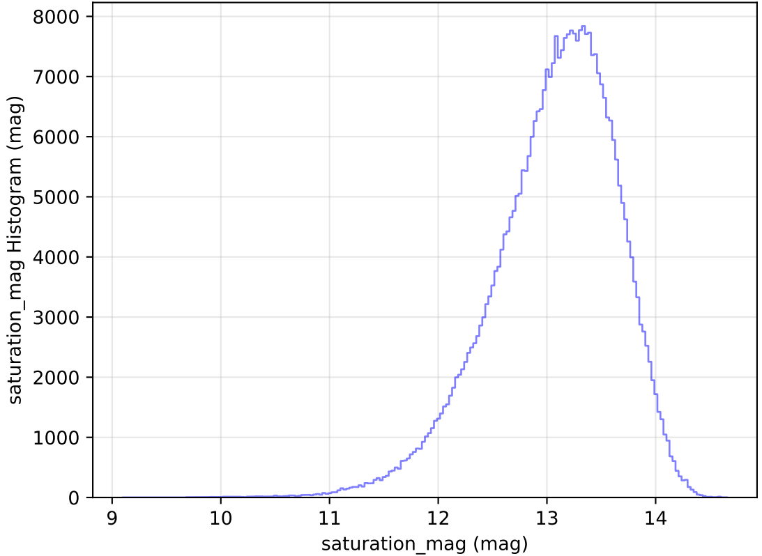
internal_u_expt38_nscale1.5v3.4_10yrs WFD y band: saturation_mag Histogram
