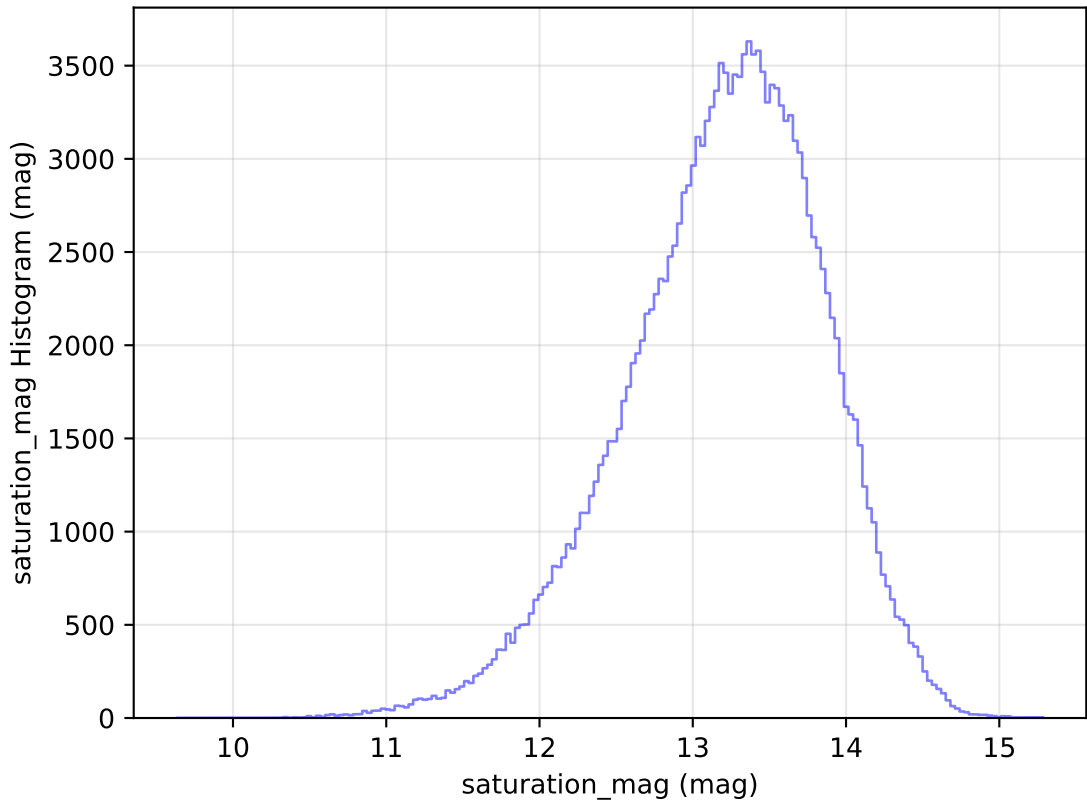
internal_u_expt38_nscale1.5v3.4_10yrs WFD u band: saturation_mag Histogram
