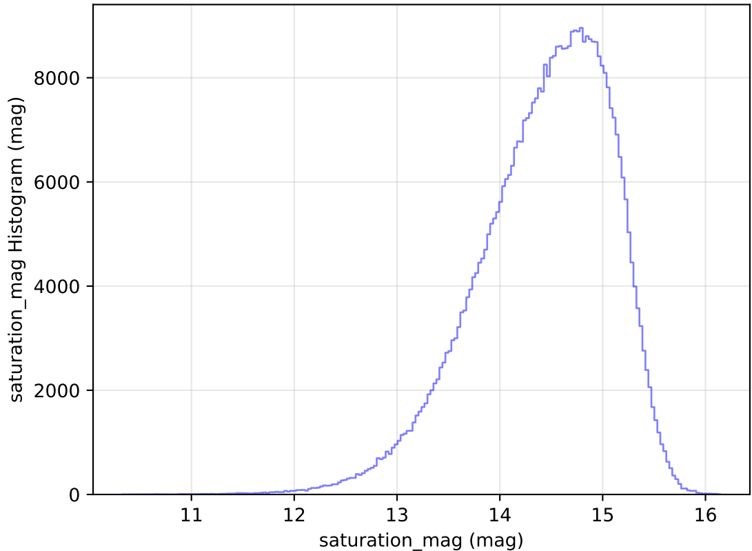
internal_u_expt38_nscale1.5v3.4_10yrs WFD i band: saturation_mag Histogram
