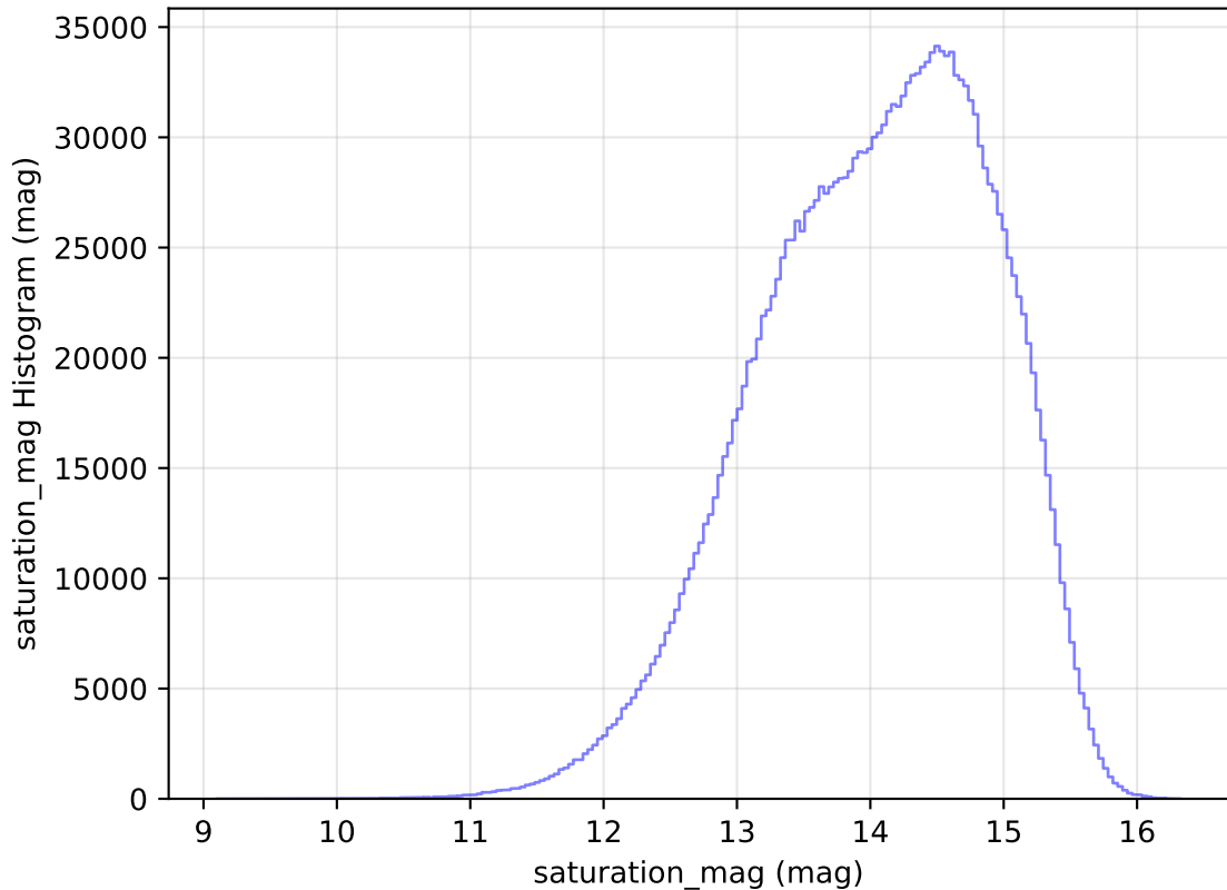
internal_u_expt38_nscale1.5v3.4_10yrs WFD all bands: saturation_mag Histogram
