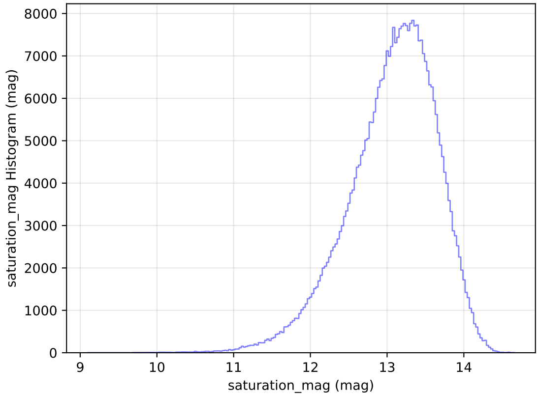
internal_u_expt38_nscale1.5v3.4_10yrs All sky y band: saturation_mag Histogram
