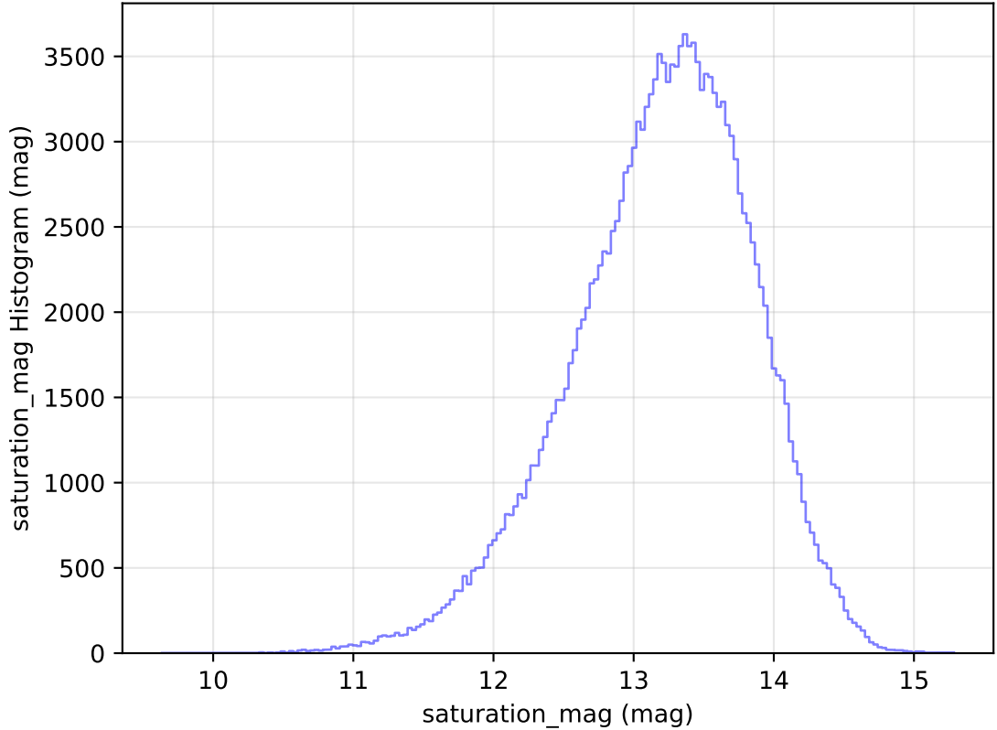
internal_u_expt38_nscale1.5v3.4_10yrs All sky u band: saturation_mag Histogram
