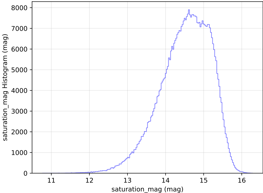
internal_u_expt38_nscale1.5v3.4_10yrs All sky r band: saturation_mag Histogram
