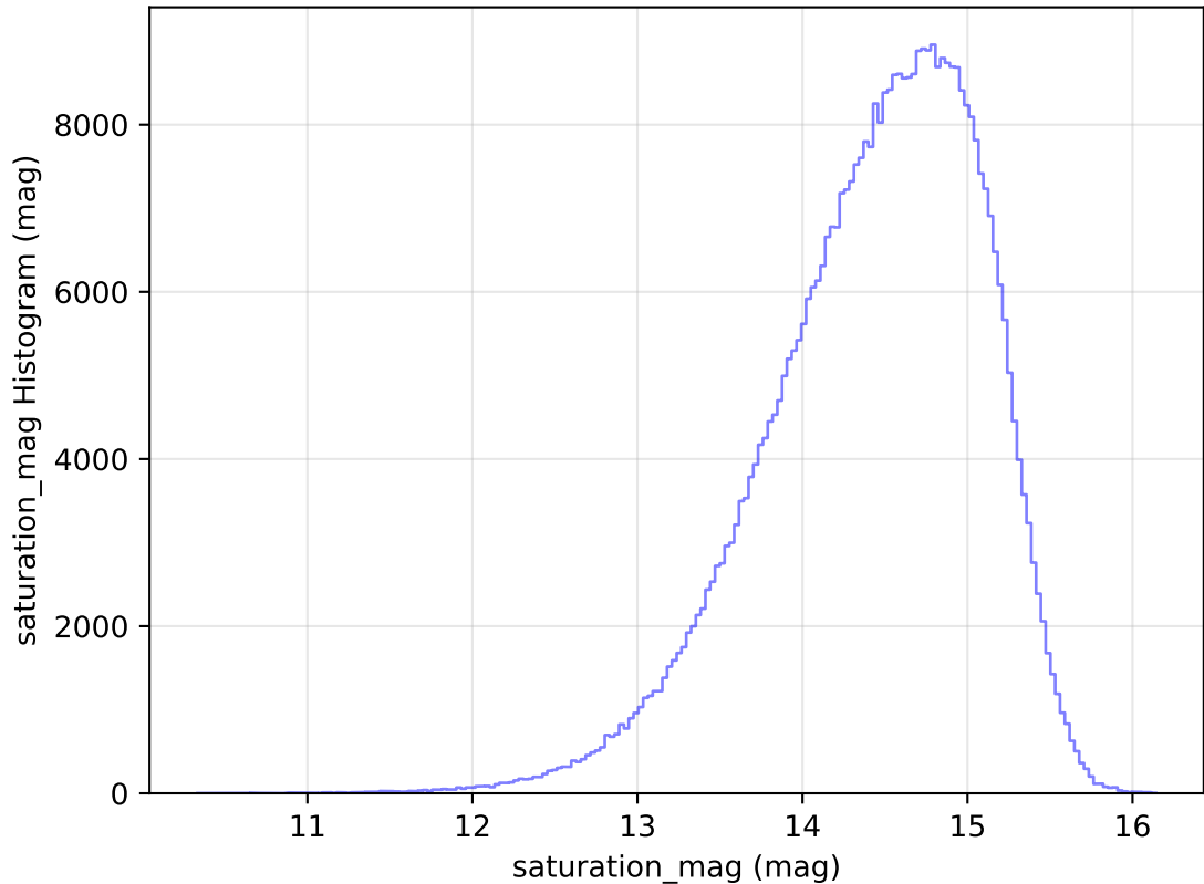
internal_u_expt38_nscale1.5v3.4_10yrs All sky i band: saturation_mag Histogram
