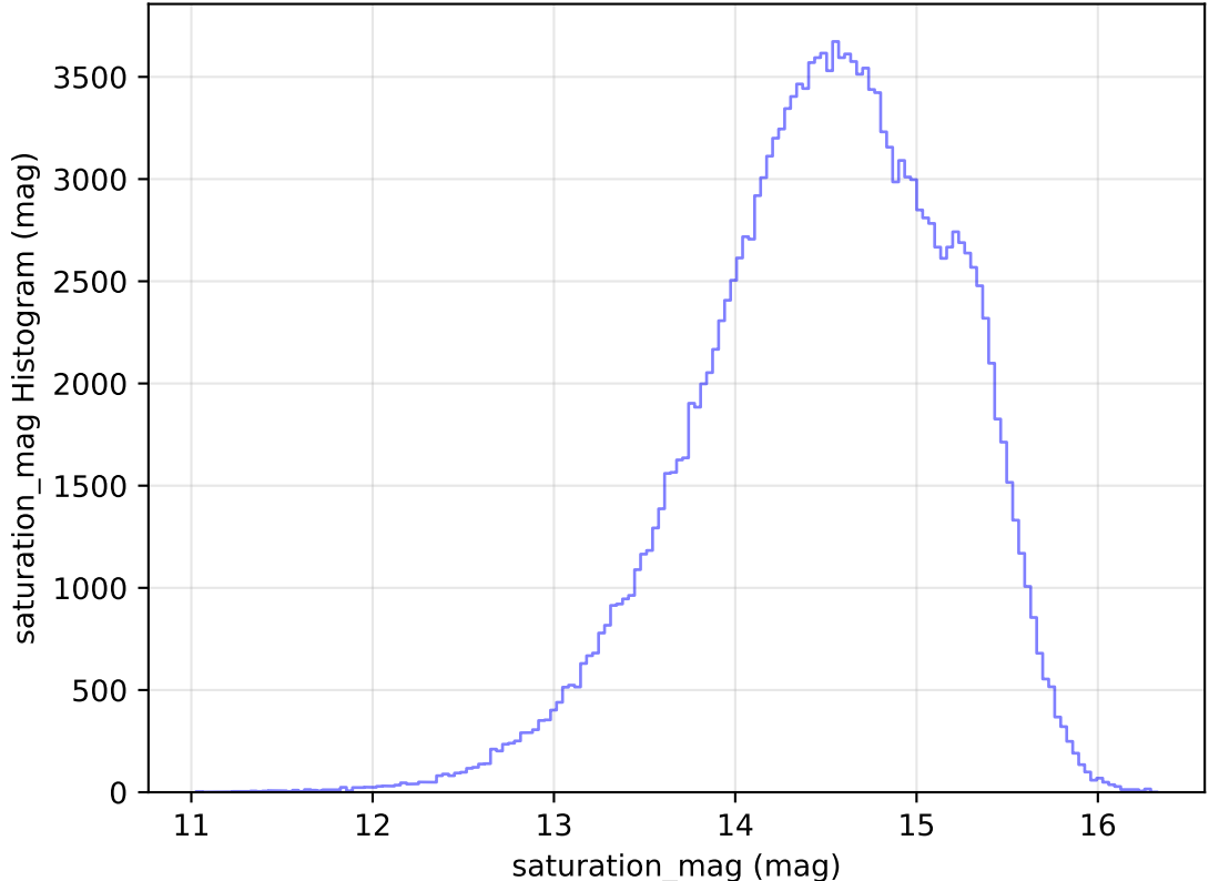
internal_u_expt38_nscale1.5v3.4_10yrs All sky g band: saturation_mag Histogram
