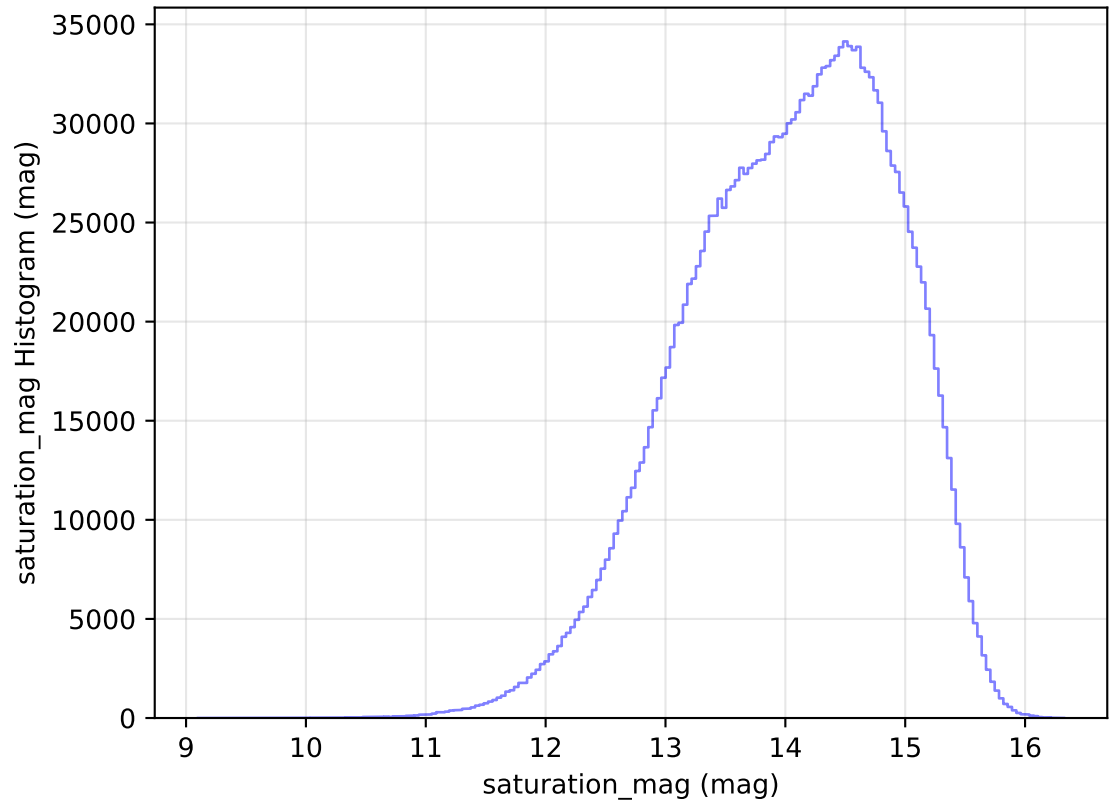
internal_u_expt38_nscale1.5v3.4_10yrs All sky all bands: saturation_mag Histogram
