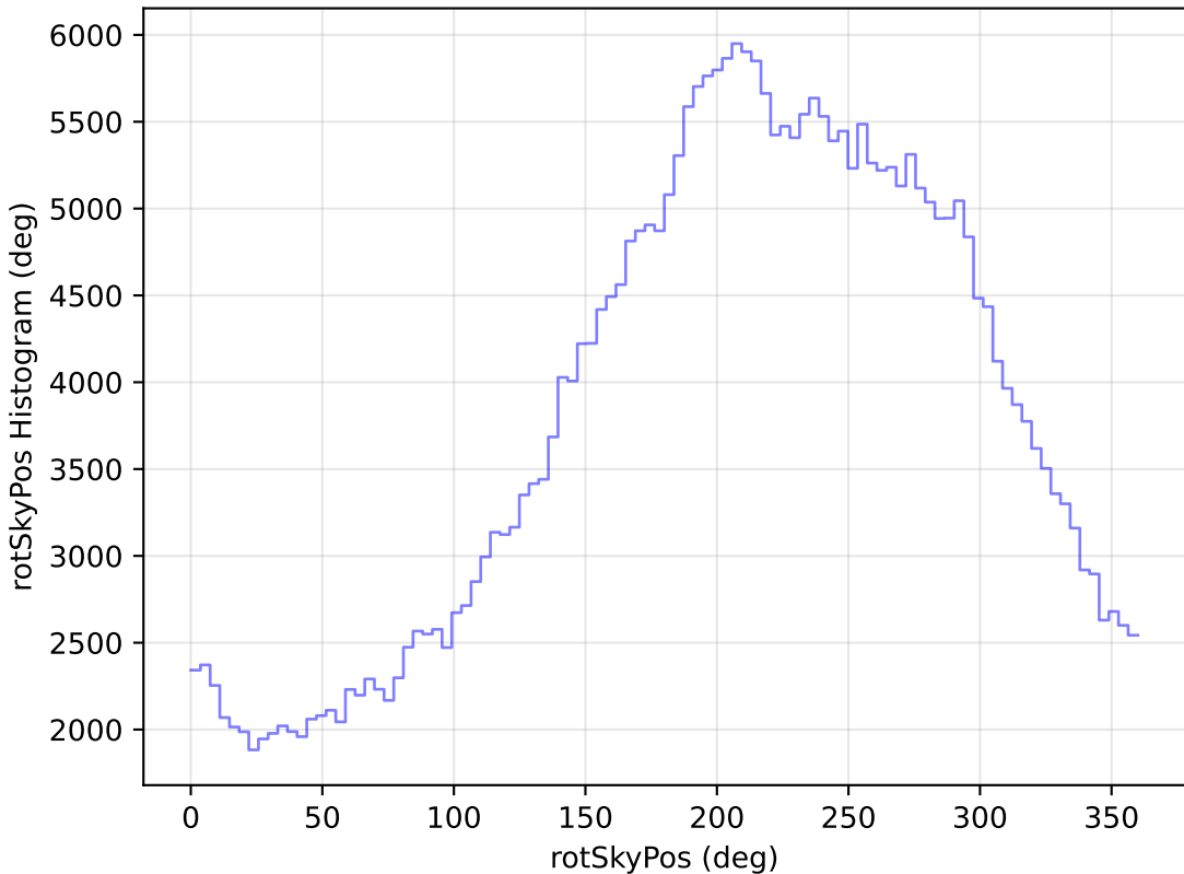
internal_u_expt38_nscale1.5v3.4_10yrs WFD y band: rotSkyPos Histogram
