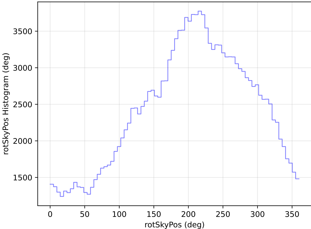
internal_u_expt38_nscale1.5v3.4_10yrs WFD u band: rotSkyPos Histogram
