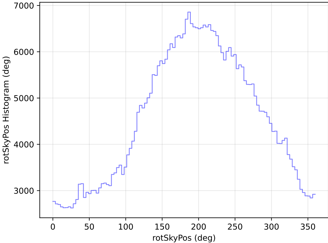
internal_u_expt38_nscale1.5v3.4_10yrs WFD r band: rotSkyPos Histogram
