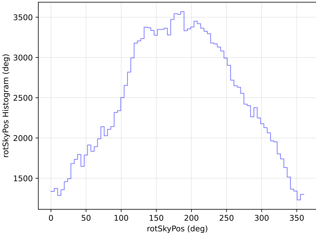
internal_u_expt38_nscale1.5v3.4_10yrs WFD g band: rotSkyPos Histogram
