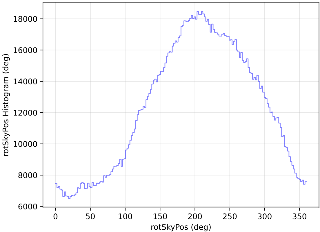
internal_u_expt38_nscale1.5v3.4_10yrs WFD all bands: rotSkyPos Histogram
