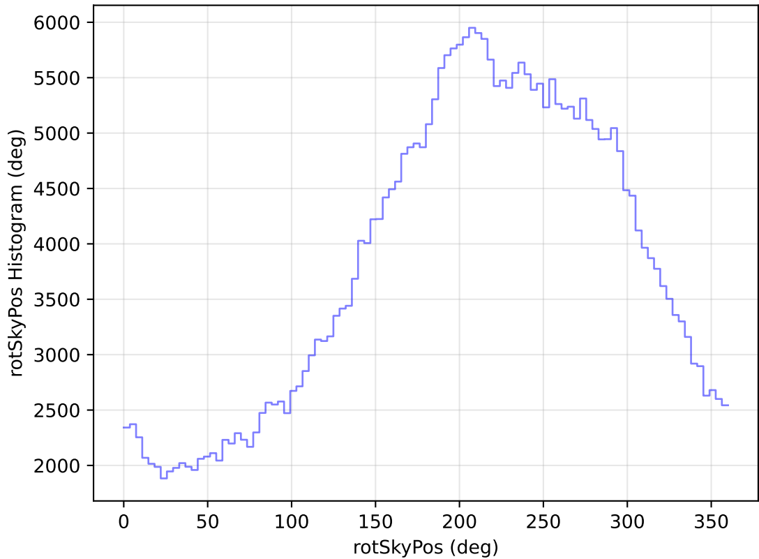
internal_u_expt38_nscale1.5v3.4_10yrs All sky y band: rotSkyPos Histogram
