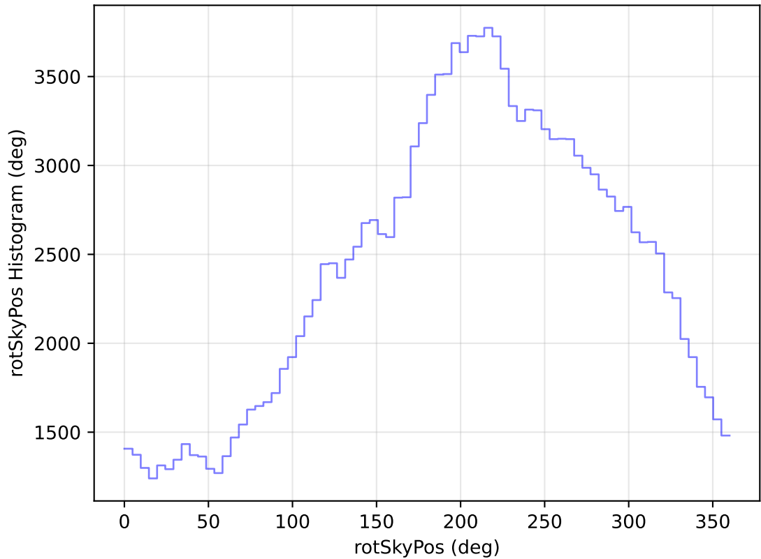
internal_u_expt38_nscale1.5v3.4_10yrs All sky u band: rotSkyPos Histogram
