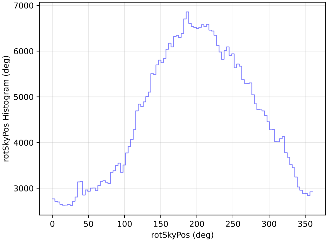
internal_u_expt38_nscale1.5v3.4_10yrs All sky r band: rotSkyPos Histogram
