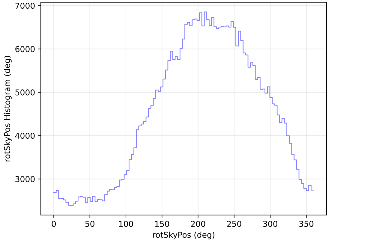
internal_u_expt38_nscale1.5v3.4_10yrs All sky i band: rotSkyPos Histogram
