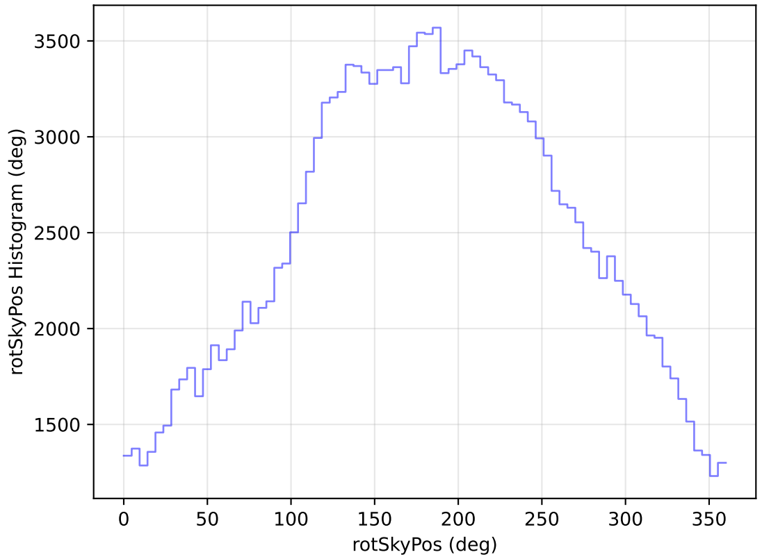
internal_u_expt38_nscale1.5v3.4_10yrs All sky g band: rotSkyPos Histogram
