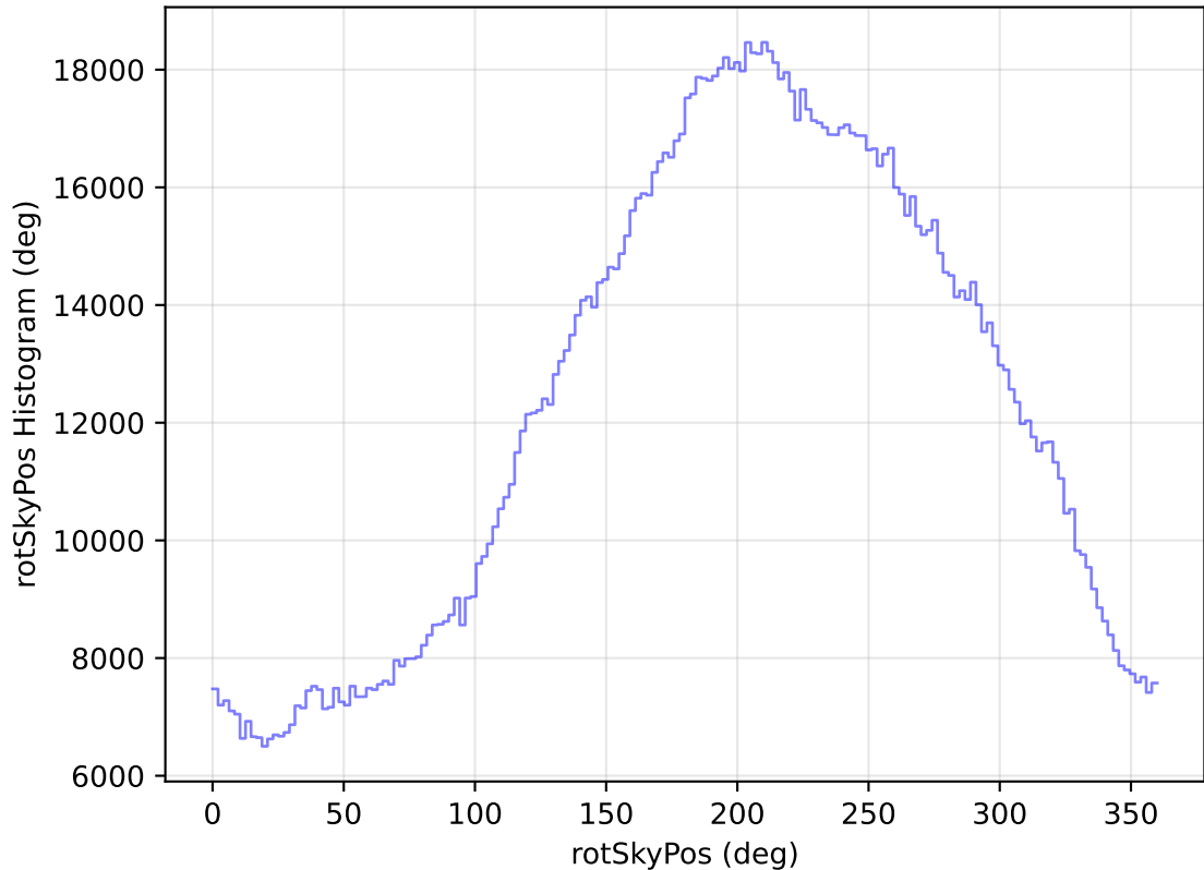
internal_u_expt38_nscale1.5v3.4_10yrs All sky all bands: rotSkyPos Histogram
