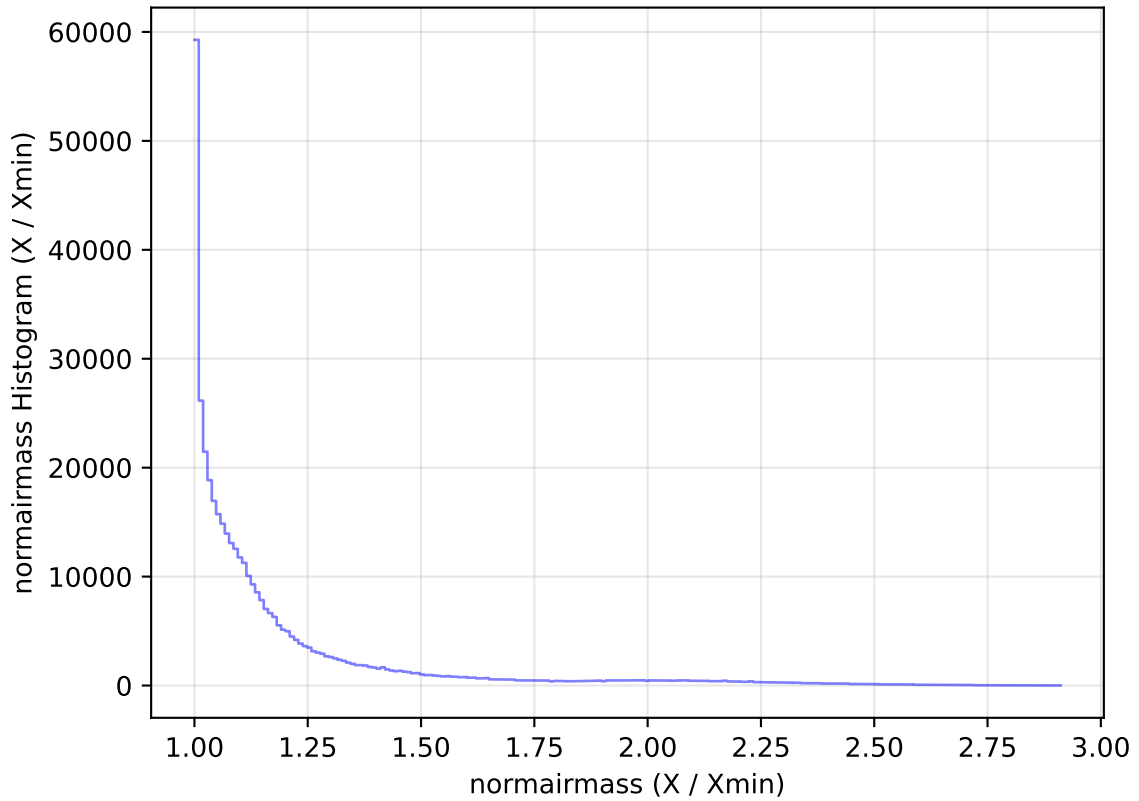
internal_u_expt38_nscale1.5v3.4_10yrs WFD z band: normairmass Histogram
