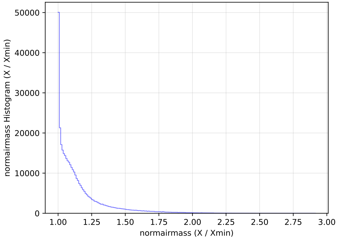
internal_u_expt38_nscale1.5v3.4_10yrs WFD y band: normairmass Histogram
