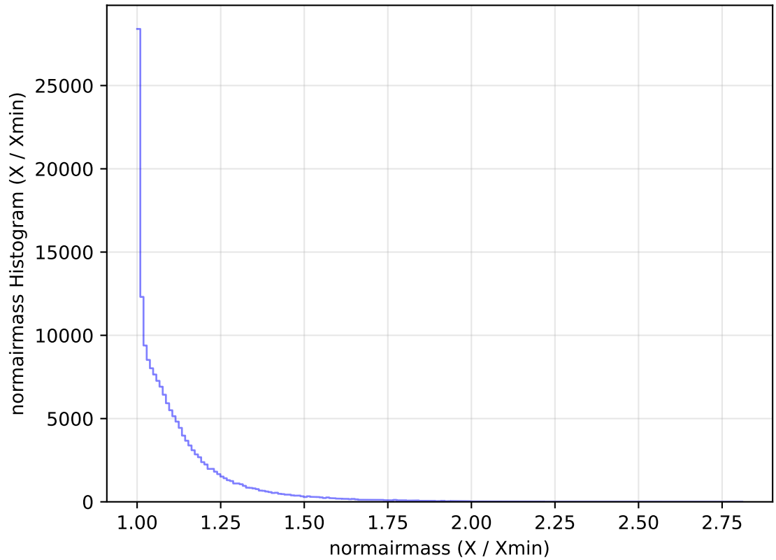
internal_u_expt38_nscale1.5v3.4_10yrs WFD u band: normairmass Histogram
