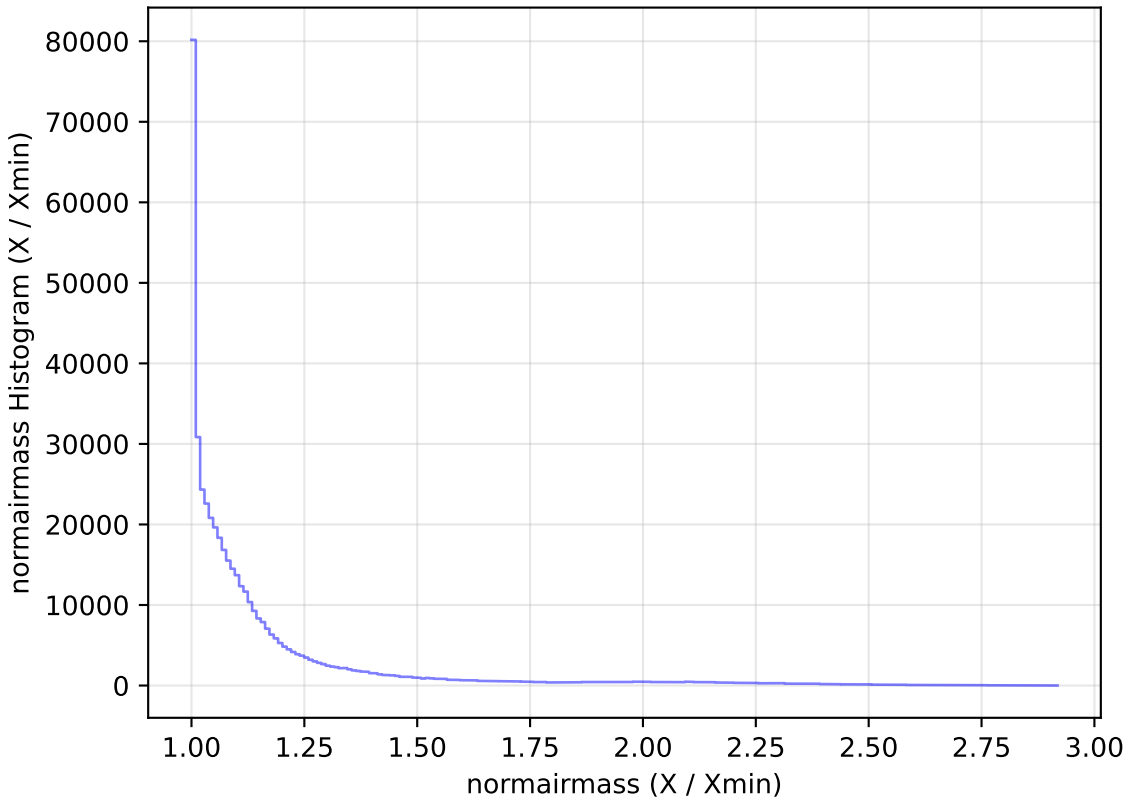
internal_u_expt38_nscale1.5v3.4_10yrs WFD i band: normairmass Histogram
