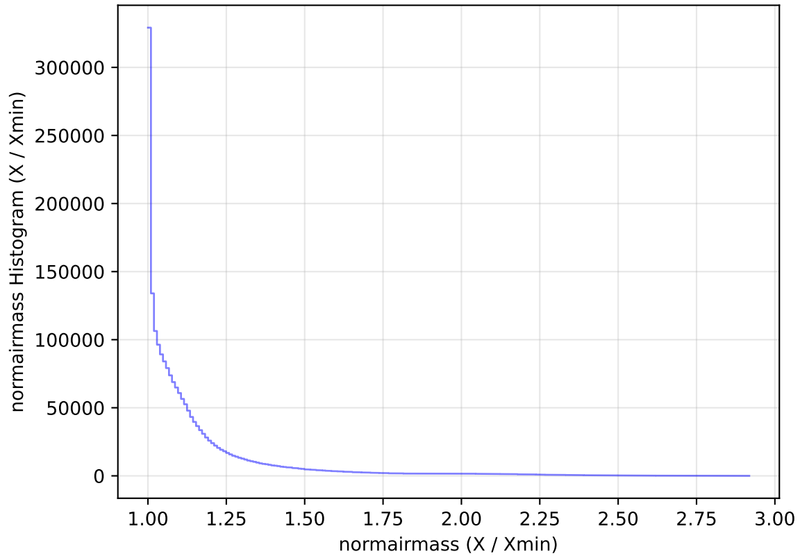
internal_u_expt38_nscale1.5v3.4_10yrs WFD all bands: normairmass Histogram
