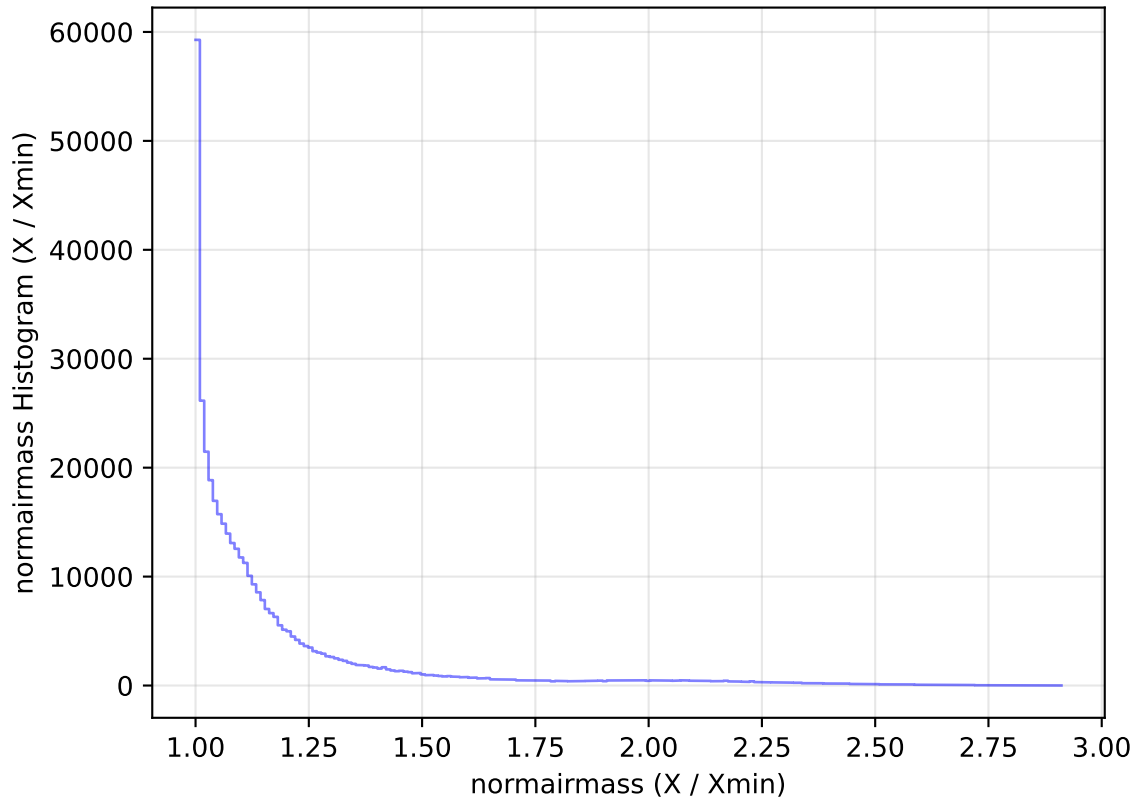
internal_u_expt38_nscale1.5v3.4_10yrs All sky z band: normairmass Histogram
