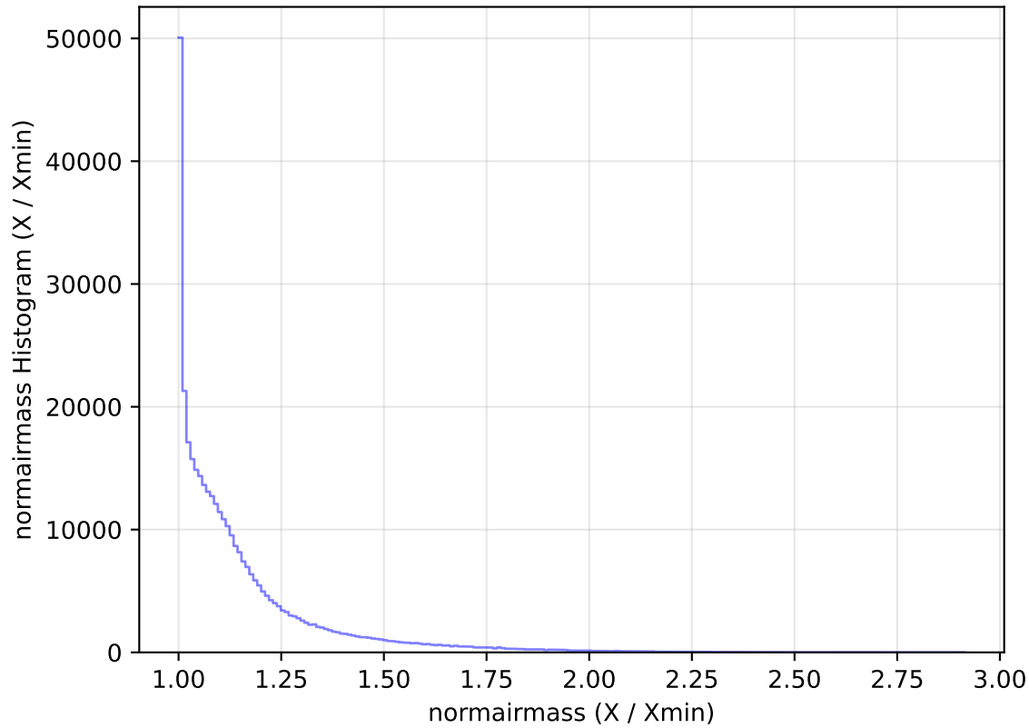
internal_u_expt38_nscale1.5v3.4_10yrs All sky y band: normairmass Histogram
