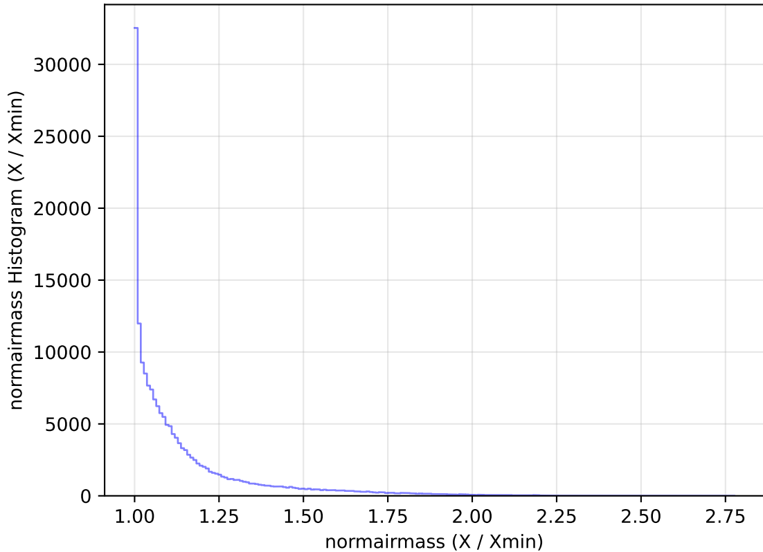
internal_u_expt38_nscale1.5v3.4_10yrs All sky g band: normairmass Histogram
