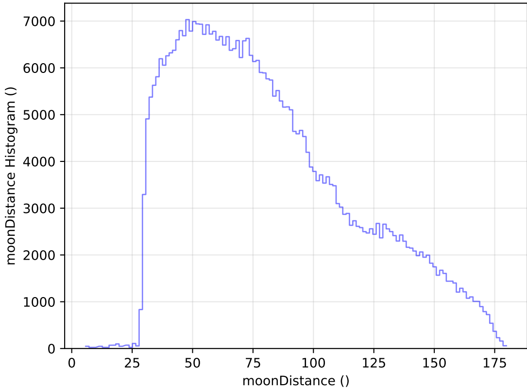
internal_u_expt38_nscale1.5v3.4_10yrs WFD z band: moonDistance Histogram
