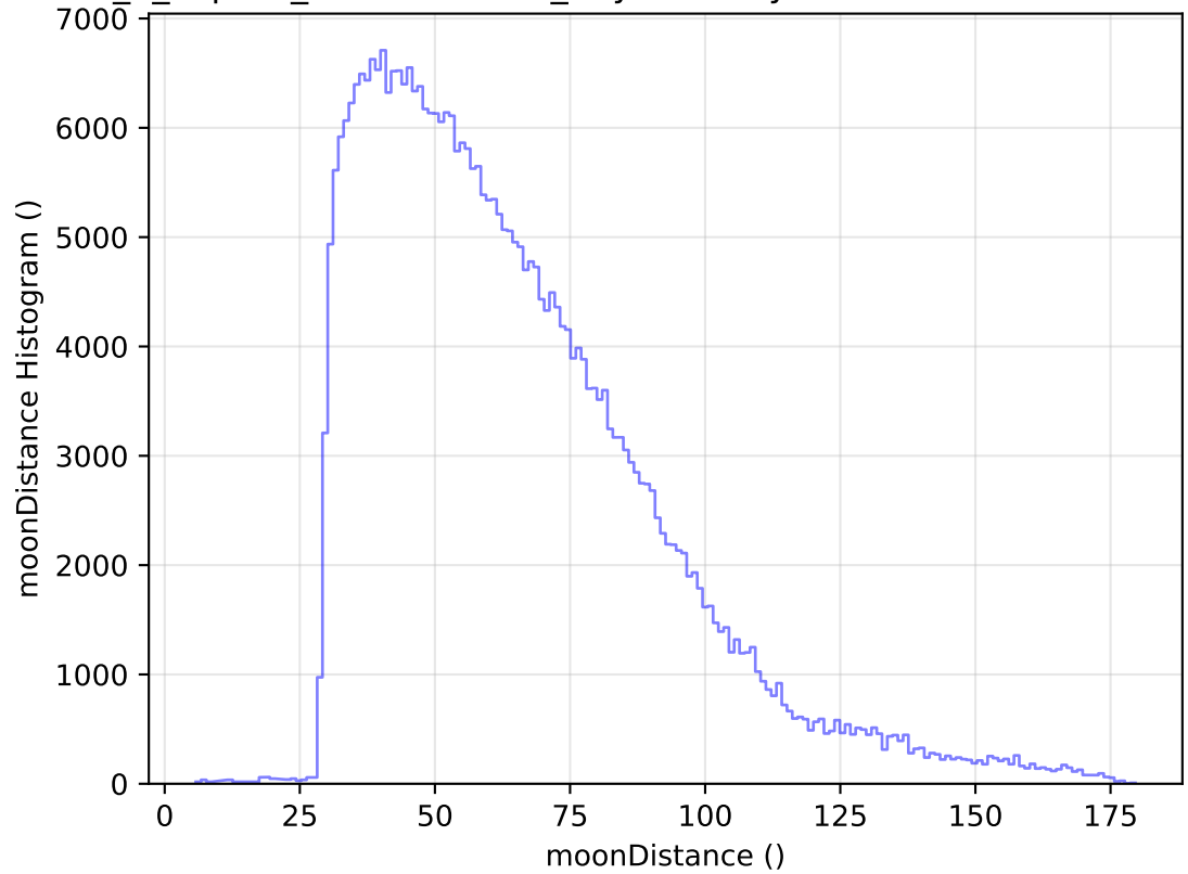
internal_u_expt38_nscale1.5v3.4_10yrs WFD y band: moonDistance Histogram
