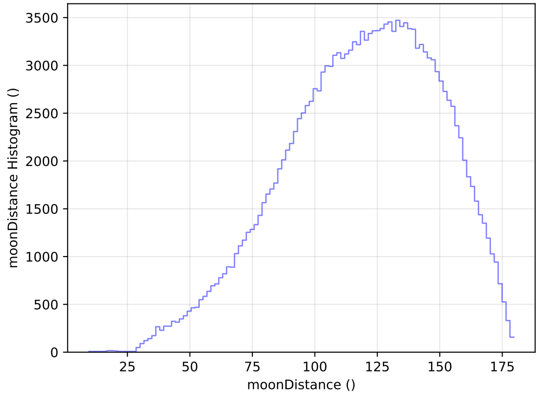
internal_u_expt38_nscale1.5v3.4_10yrs WFD u band: moonDistance Histogram
