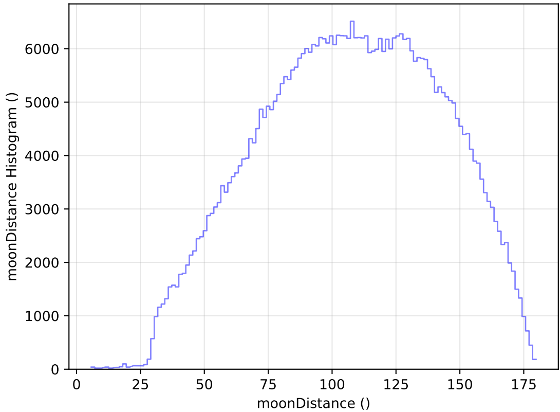
internal_u_expt38_nscale1.5v3.4_10yrs WFD r band: moonDistance Histogram
