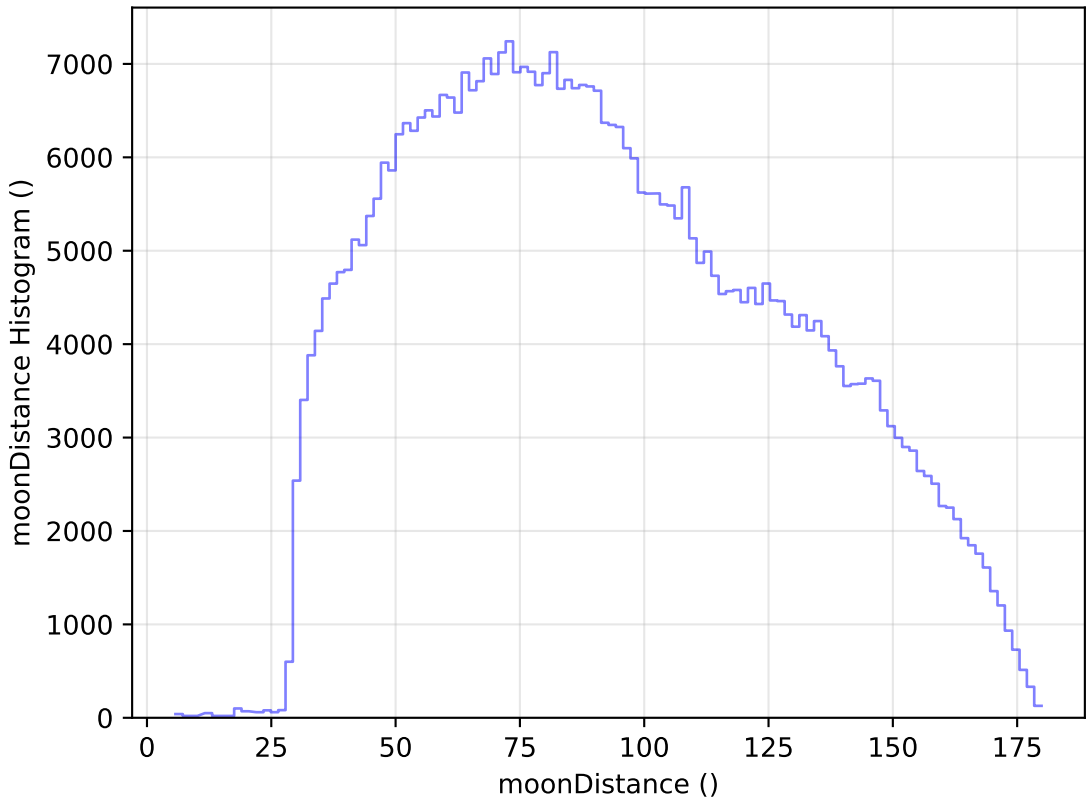
internal_u_expt38_nscale1.5v3.4_10yrs WFD i band: moonDistance Histogram
