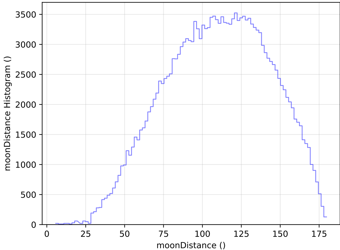
internal_u_expt38_nscale1.5v3.4_10yrs WFD g band: moonDistance Histogram
