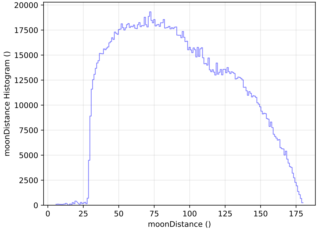
internal_u_expt38_nscale1.5v3.4_10yrs WFD all bands: moonDistance Histogram
