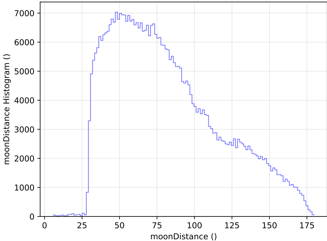
internal_u_expt38_nscale1.5v3.4_10yrs All sky z band: moonDistance Histogram
