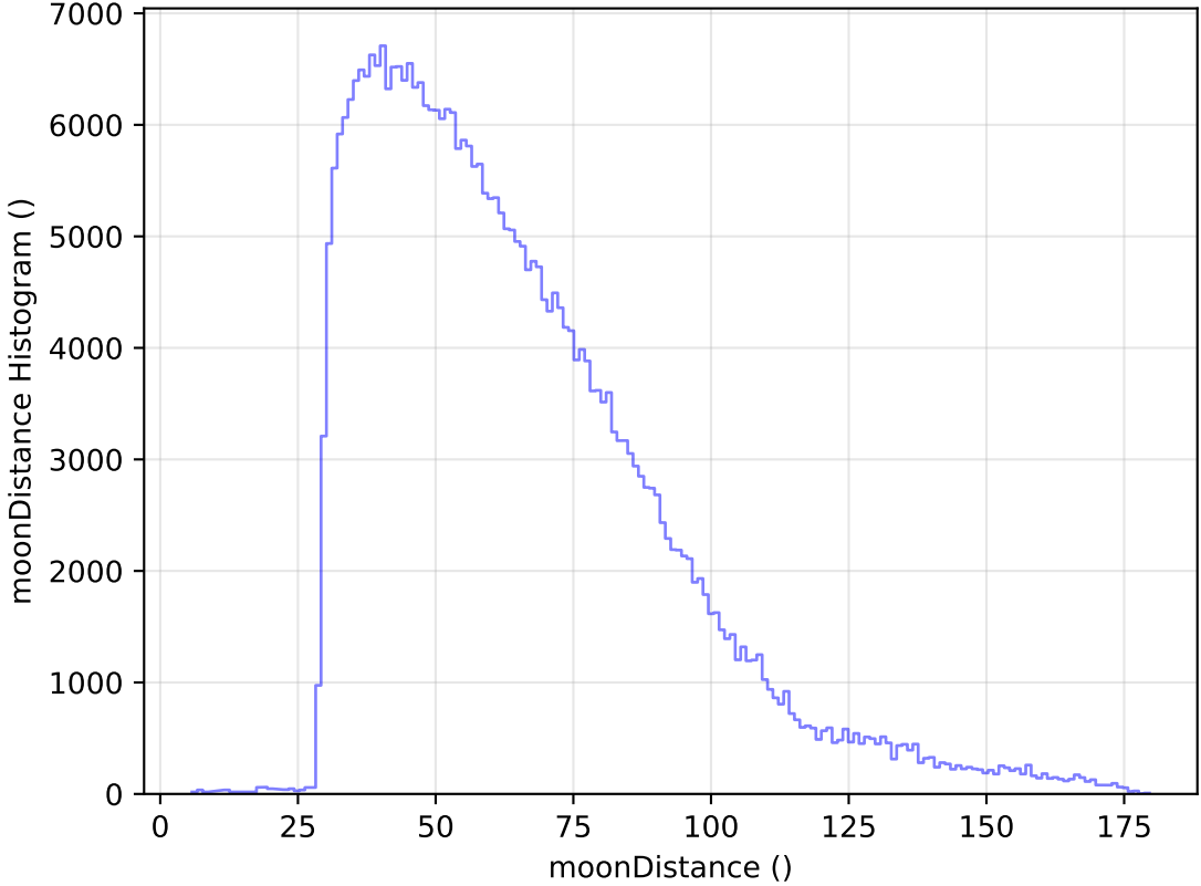
internal_u_expt38_nscale1.5v3.4_10yrs All sky y band: moonDistance Histogram
