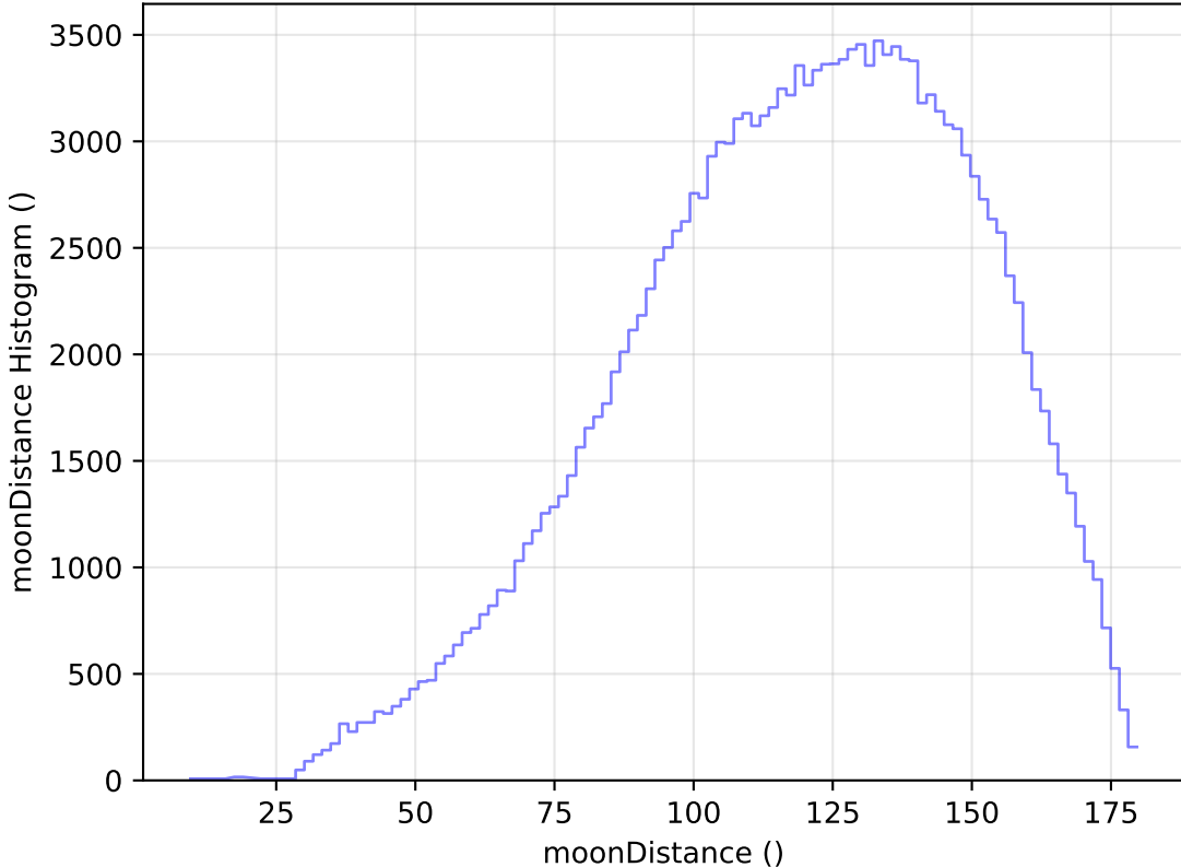
internal_u_expt38_nscale1.5v3.4_10yrs All sky u band: moonDistance Histogram
