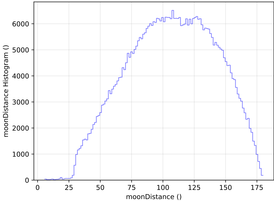
internal_u_expt38_nscale1.5v3.4_10yrs All sky r band: moonDistance Histogram
