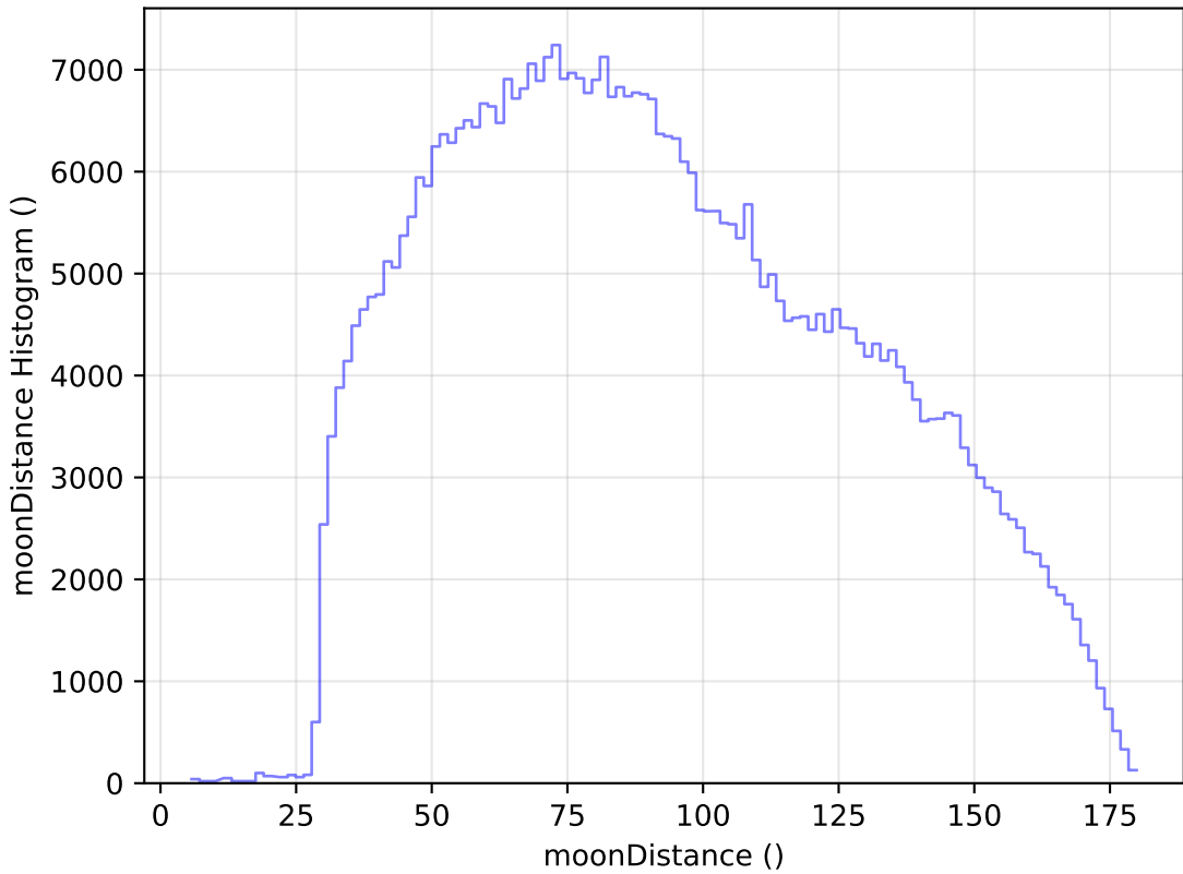
internal_u_expt38_nscale1.5v3.4_10yrs All sky i band: moonDistance Histogram
