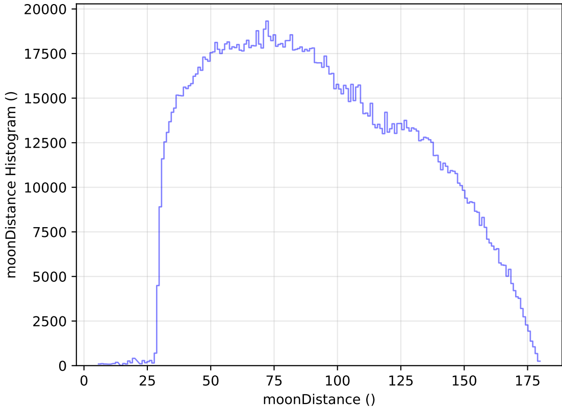
internal_u_expt38_nscale1.5v3.4_10yrs All sky all bands: moonDistance Histogram
