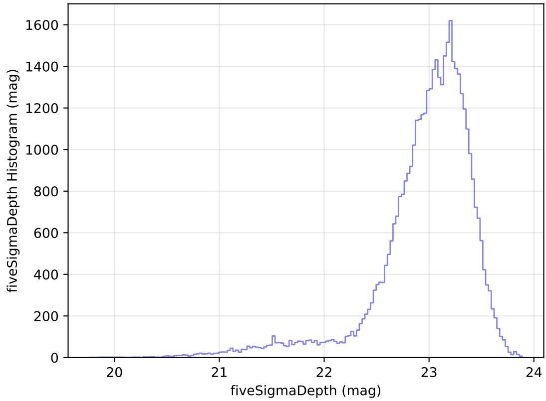
internal_u_expt38_nscale1.5v3.4_10yrs Yr 1 z band: fiveSigmaDepth Histogram
