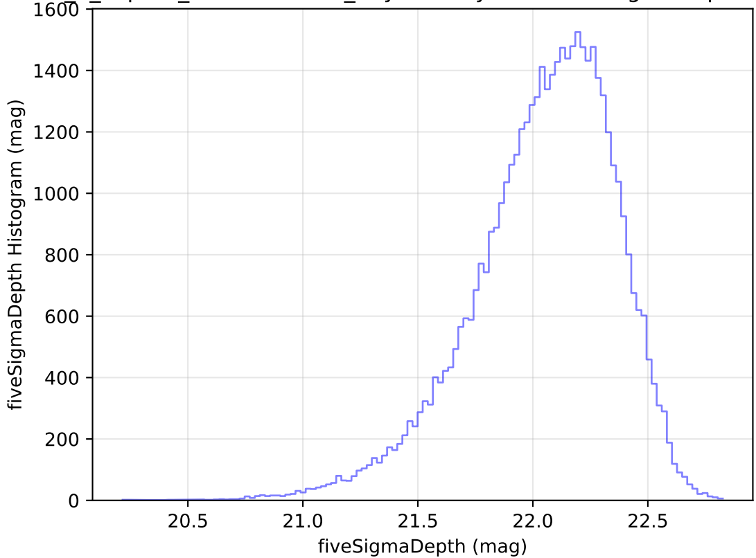
internal_u_expt38_nscale1.5v3.4_10yrs Yr 1 y band: fiveSigmaDepth Histogram
