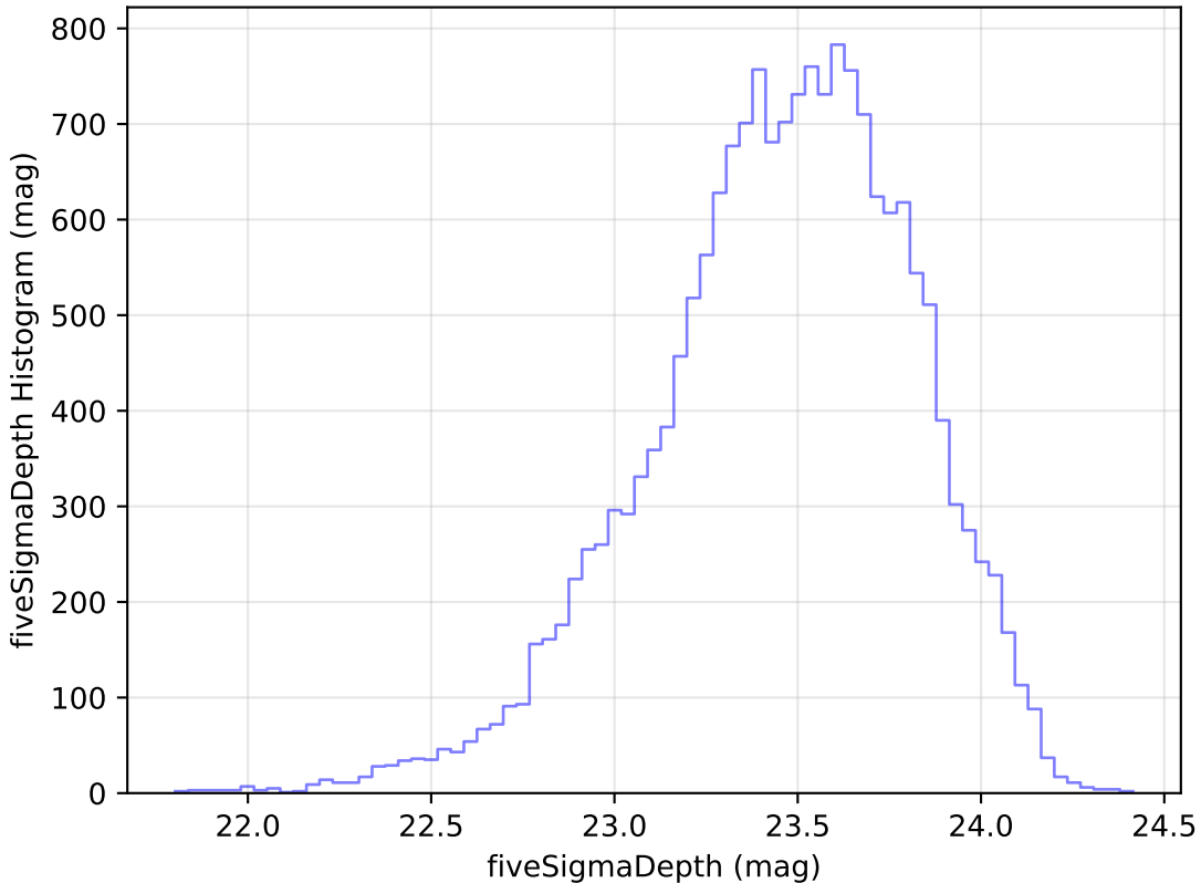
internal_u_expt38_nscale1.5v3.4_10yrs Yr 1 u band: fiveSigmaDepth Histogram
