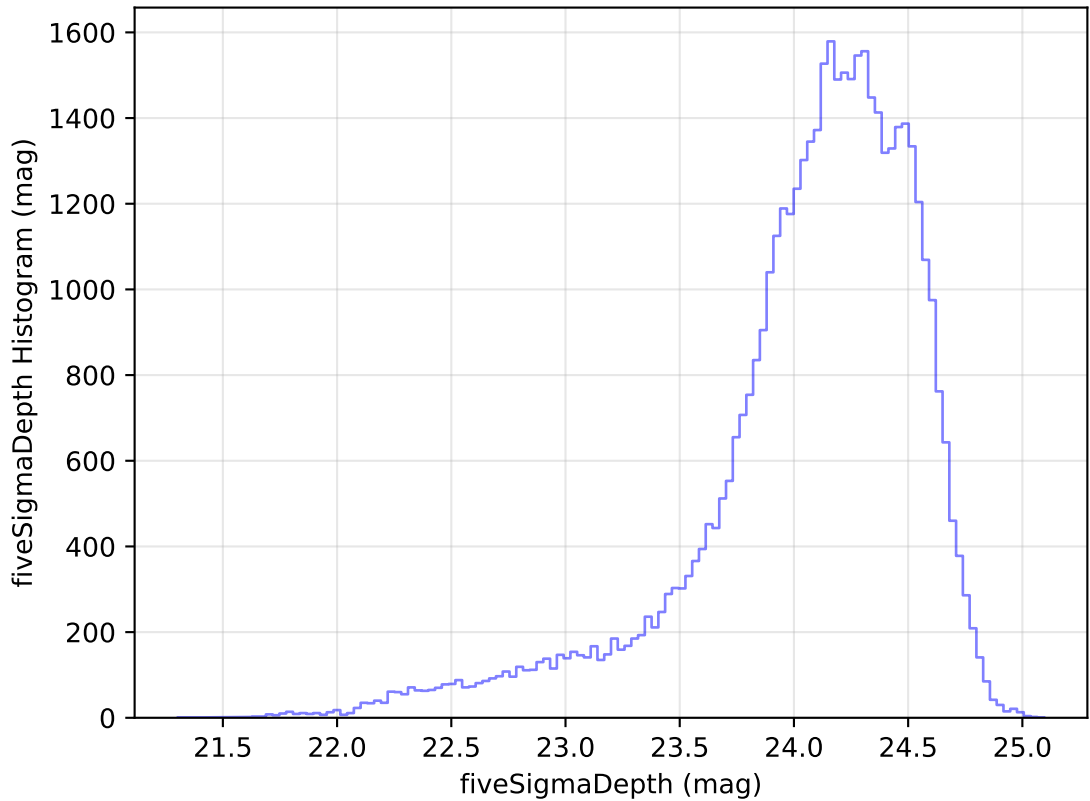
internal_u_expt38_nscale1.5v3.4_10yrs Yr 1 r band: fiveSigmaDepth Histogram
